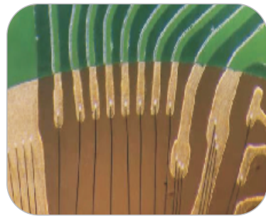
Wire bonding
